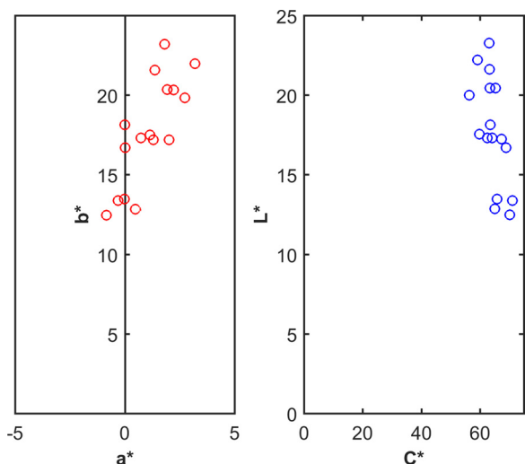
Fig. 5. The CIELAB a^*-b^* (left) and L^*-C^* (right) coordinates of the 16 tabs in the Vita Classic Shade Guide [22]. Note that the changes in color attributes tend to be correlated (for example, L^* increases as C^* decreases).
