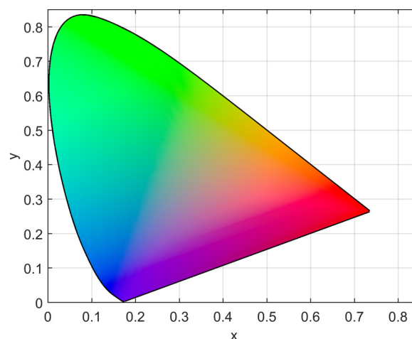
Fig. 4. The CIE chromaticity diagram.
